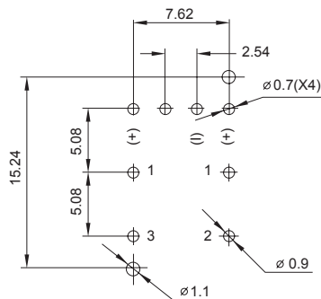
P.C.B.Mounting Holes
